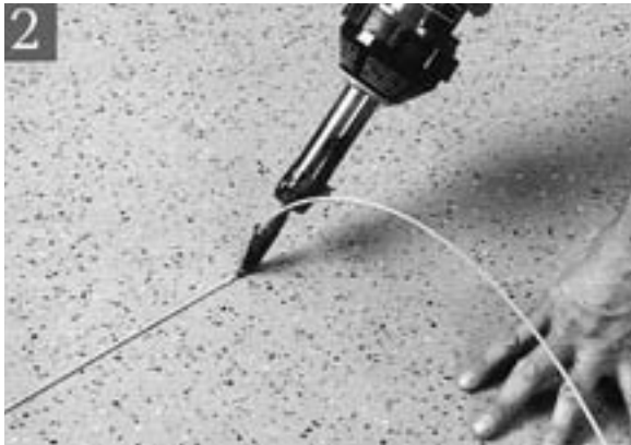
2. Hot weld joints using the hot air welding gun, speed nozzle and the appropriate colour of weldrod.
