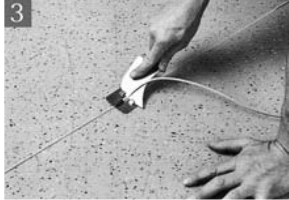
3. Remove the surplus weldrod initially using a sledge and spatula.
